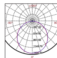
NLED4204/40W/66
