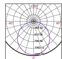
NLED4204/40W/123
